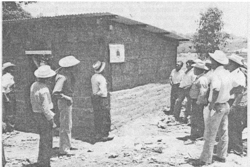
FIG 9. Model houses of the OXFAM/World Neighbors program. Note the insertion of adobe blocks within the sawn timber frame in the top photograph.
