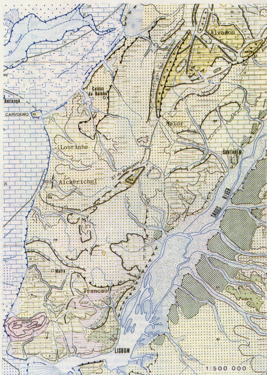
Fig.1-Geomorphological map of Estremadura (from D. B. FERREIRA, 1981)
