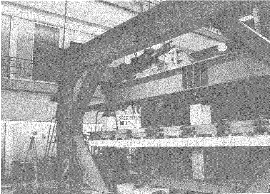
FIGURE 2-7 Specimen DNY_2 in Testing Frame
