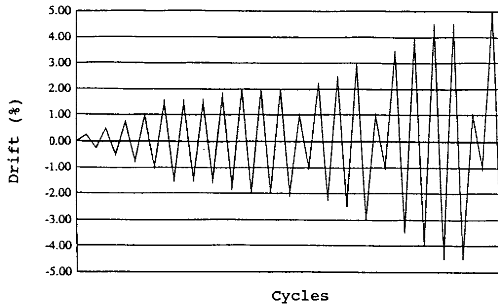
FIGURE 2-9 Lateral Displacement Routine
